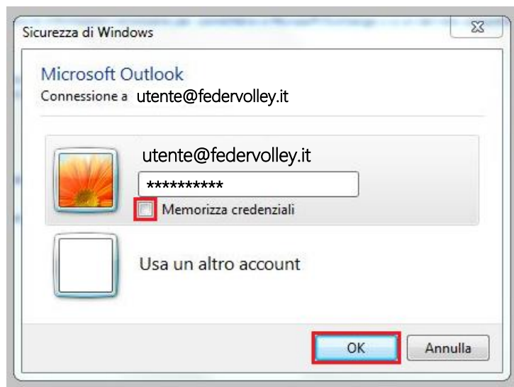
Figura 25 – Verifica User
